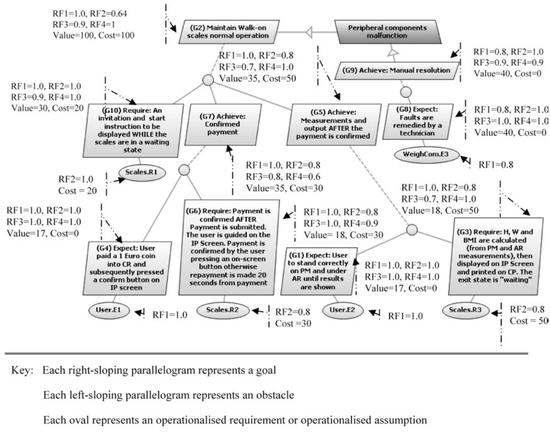
Fig. 3 WeighCom: annotated goal graph for root goal 'Maintain walk-on scales normal operation'
