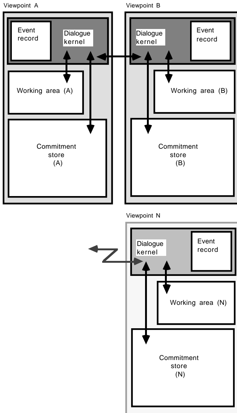
Figure 1 Block diagram of viewpoint architecture
